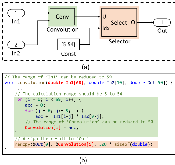
Fig. 1. Sample model to illustrate the motivation of our work. The green part represents the code generated from the Convolution block. The orange part represents the code generated from the Selector block. The variables highlighted in red indicate those whose memory usage can be reduced. (a) Convolution model. (b) Generated code.
