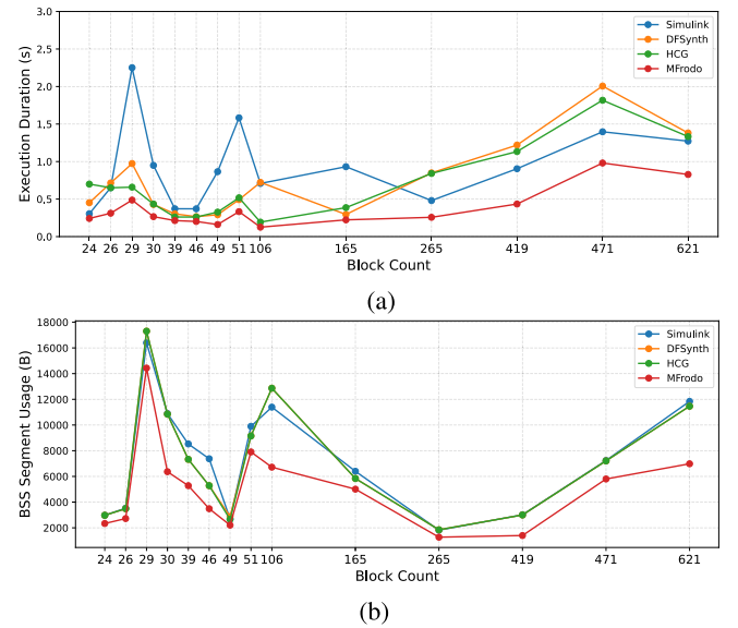
Fig. 7. Trends in execution duration and BSS segment usage as the block count increased. (a) Trend in execution duration with increasing block count. (b) Trend in BSS segment usage with increasing block count.
