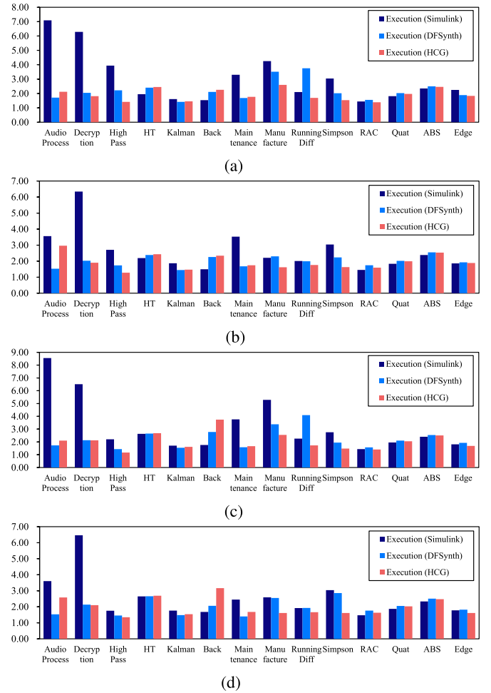
Fig. 6. Execution improvement of the code generated by MFRODO versus other code generators on ARM. (a) Execution Improvement on ARM with GCC under -O1 flag. (b) Execution Improvement on ARM with Clang under -O1 flag. (c) Execution Improvement on ARM with GCC under -O3 flag. (d) Execution Improvement on ARM with Clang under -O3 flag.
