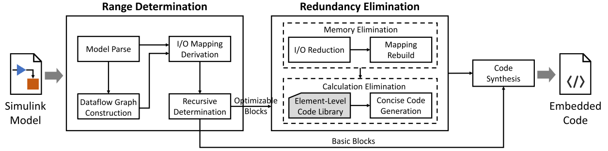
Fig. 2. Overall framework of MFRODO. 1) Range determination: MFRODO parses the target model to collect critical information. Then, MFRODO constructs the dataflow graph and derives the I/O mapping of each block. For each block, MFRODO recursively determines its precise input and output ranges as well as its subsequent blocks. 2) Redundancy elimination: For optimizable blocks, MFRODO reduces the memory space related to unnecessary calculations and records the new indices of inputs and outputs. Based on these indices, MFRODO rebuilds the I/O mappings to ensure code correctness.
