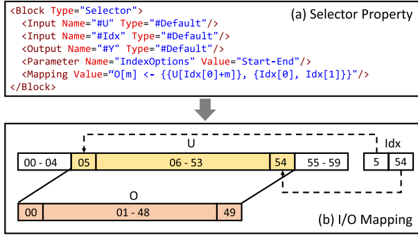
Fig. 3. Example of I/O mapping derivation. (a) Selector block's property, while (b) shows the mapping between inputs and output.
